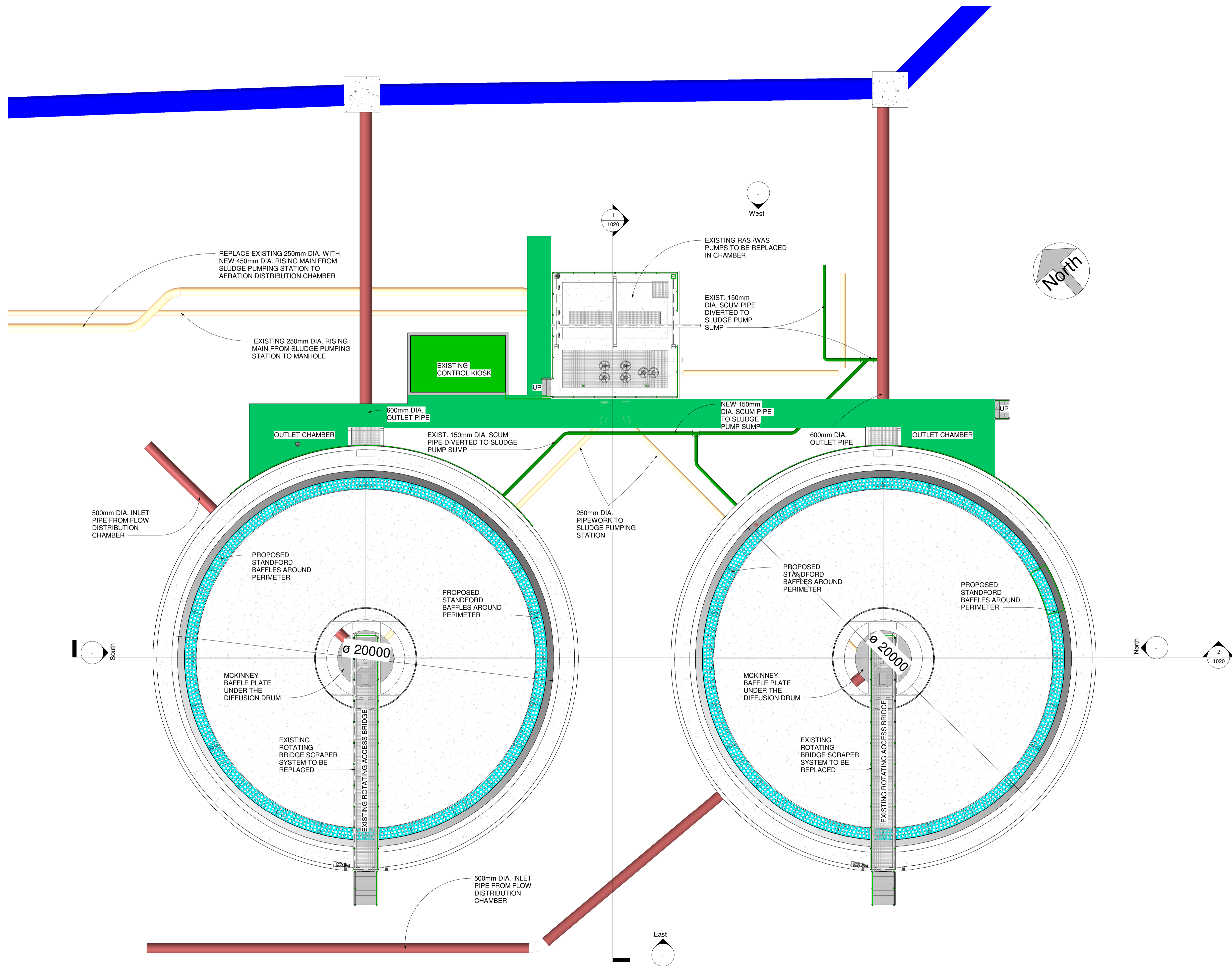
1 Clarifier Tank Plan Layout 1 : 100
